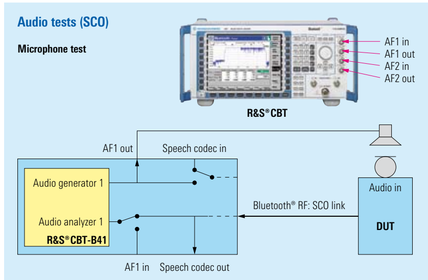
Audio measurement of a DUT microphone with the R&S® CBT-B41 option
